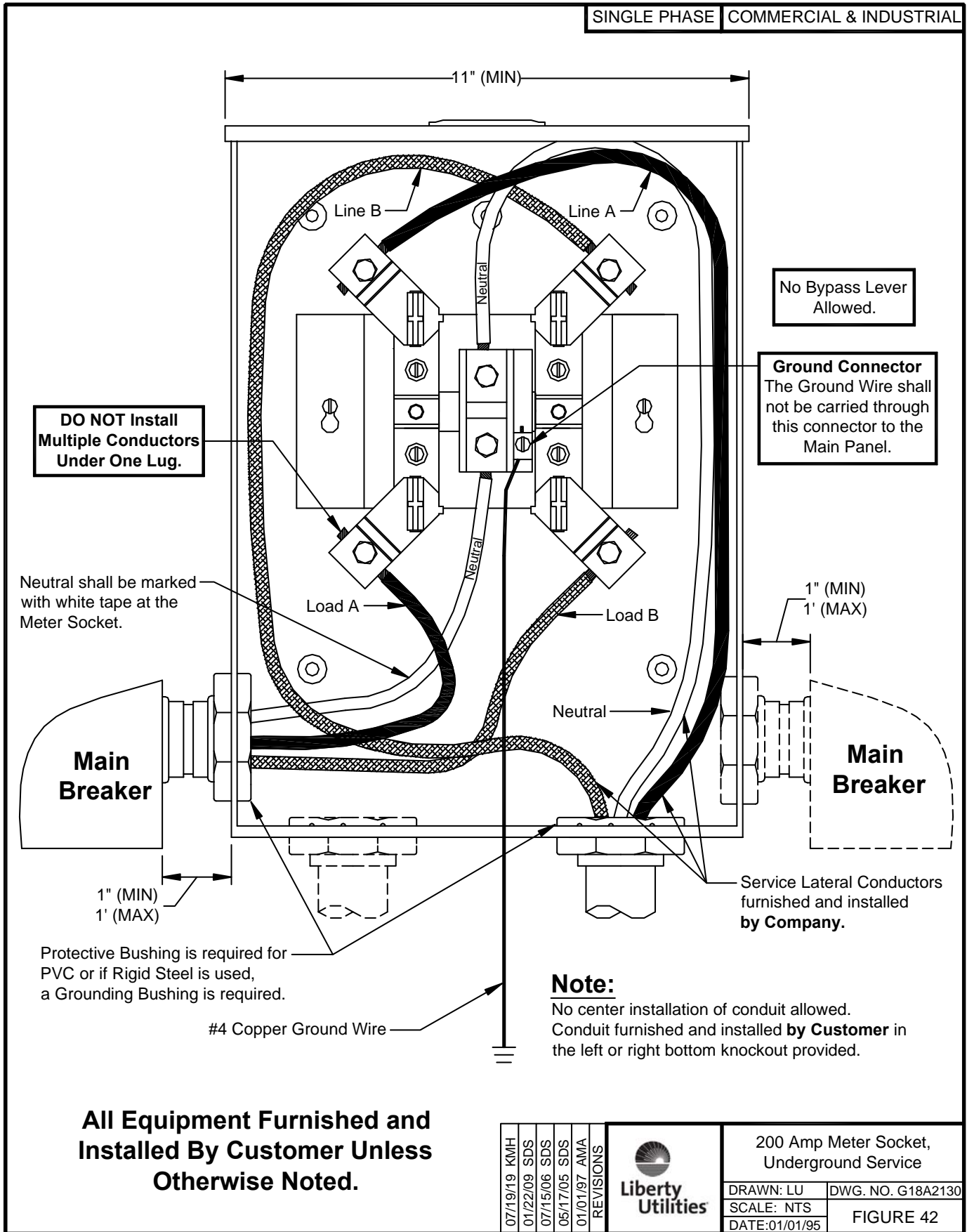
Figure 42: 200 Amp Meter Socket, Underground Service
